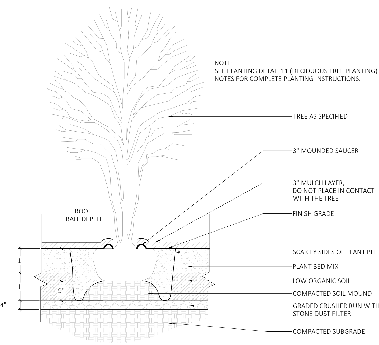
5 MULTISTEM TREE PLANTING SCALE: 1/2"=1'
